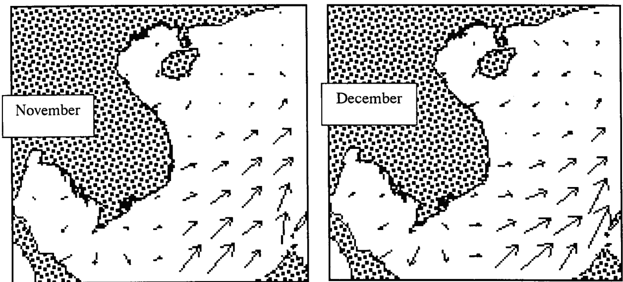
South-china sea density current patterns
